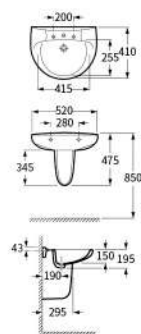
DEBBA 迪芭掛牆式面盆
