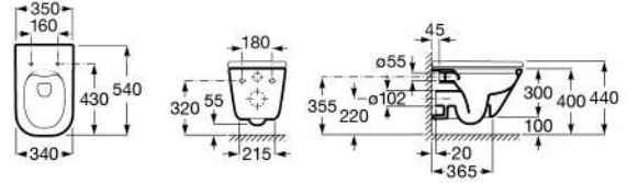
THE GAP RIMLESS 蓋普致選無圈孔掛牆馬桶
