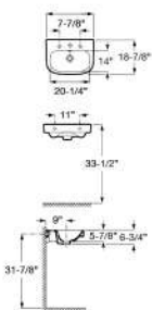
DIVERTA 碟塔掛牆式面盆
