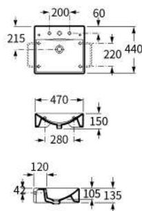
DIVERTA 碟塔掛牆式面盆
